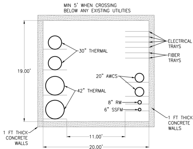
Figure 9.2. Conceptual Utilidor Section
