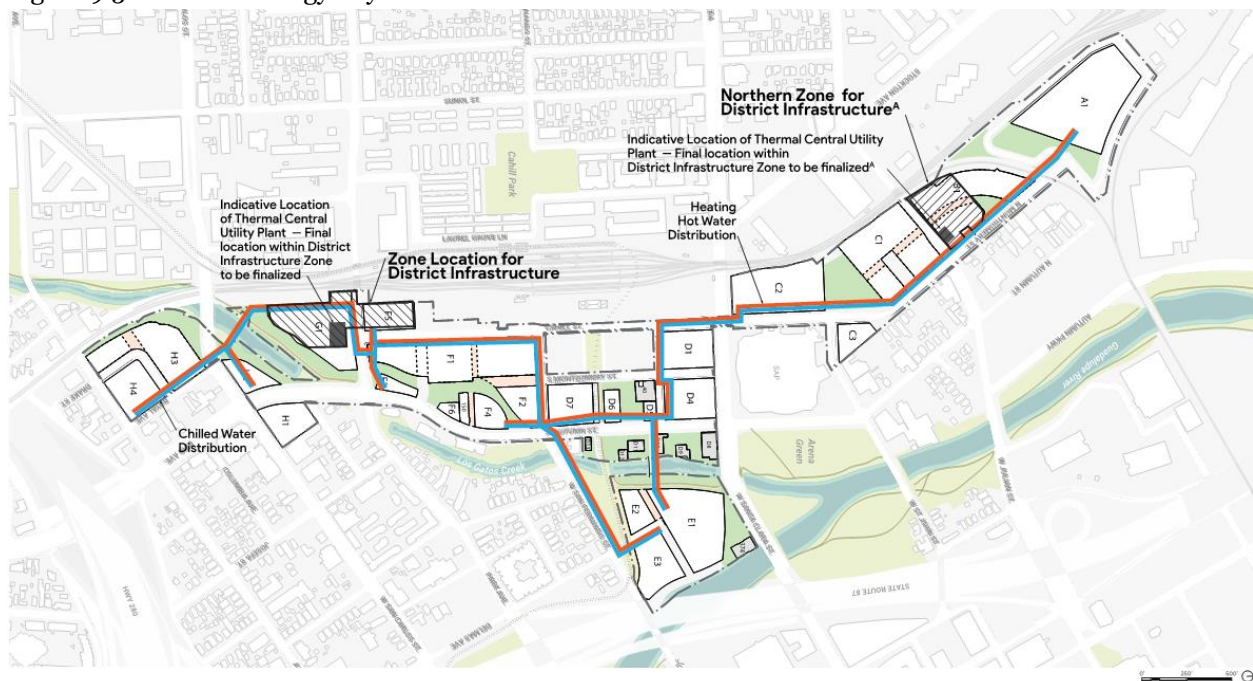
Figure 9.5. Thermal Energy Layout.
