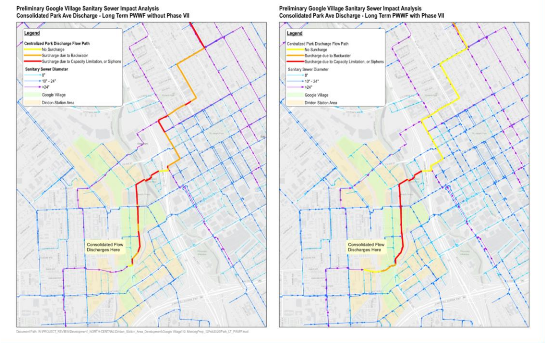
Figure 7.4. Scenario 2, One WRF with one point of connection at Park Avenue
