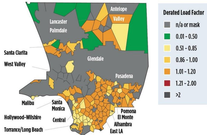
Figure 24: Map of SCE Substation Vulnerabilities to Heat Waves in 2018
