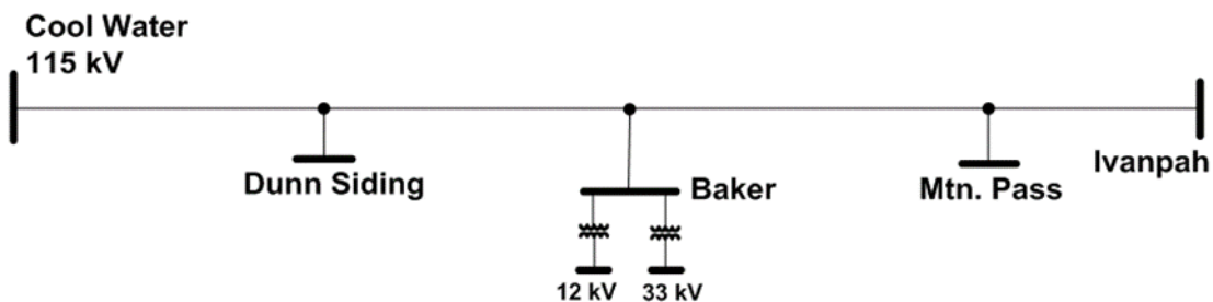
Figure 2.7-2 Proposed Configuration
