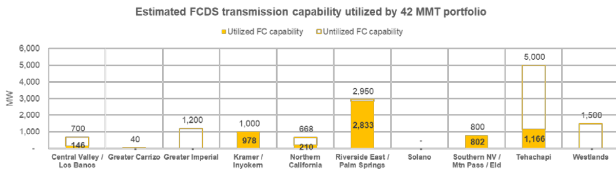
Figure 3.3-4: Utilization of FCDS transmission capability estimates
