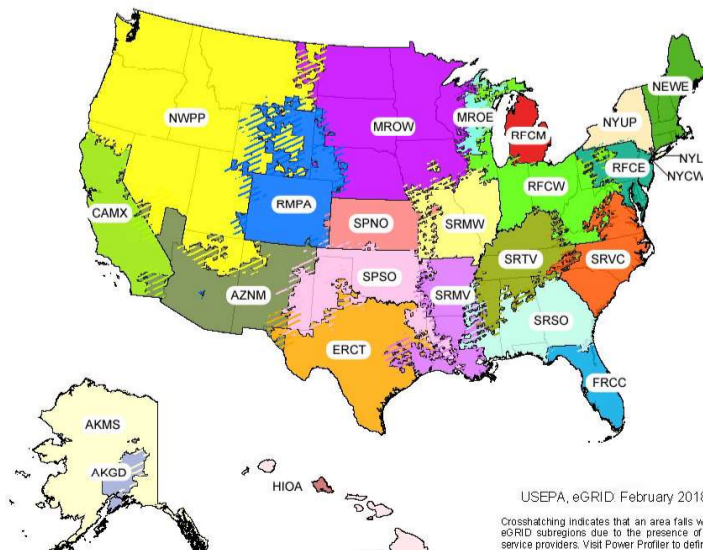
Map of eGRID Subregions
