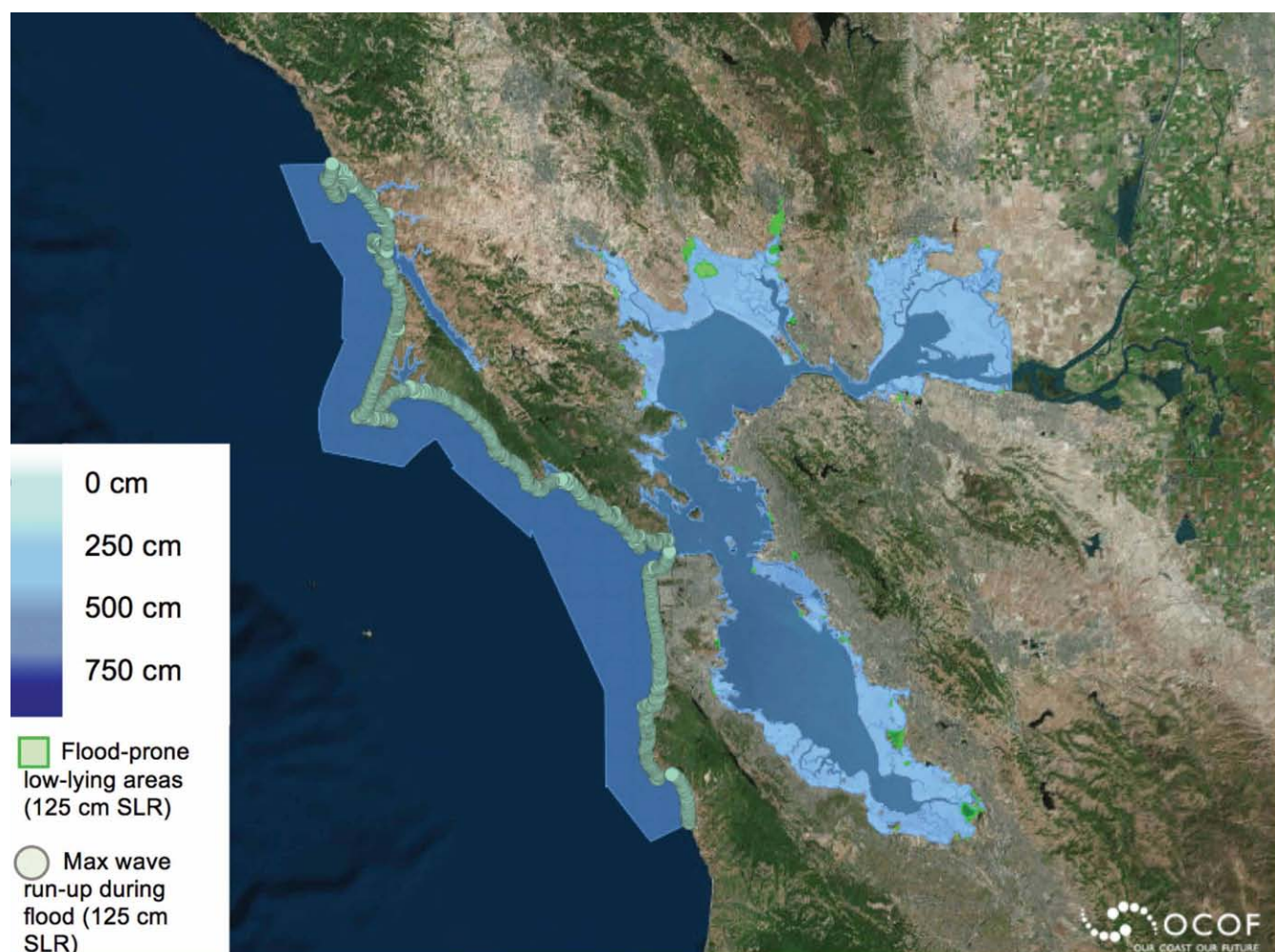
Figure 3-2. Bay Area Flooding from 4-Foot Sea-Level Rise
