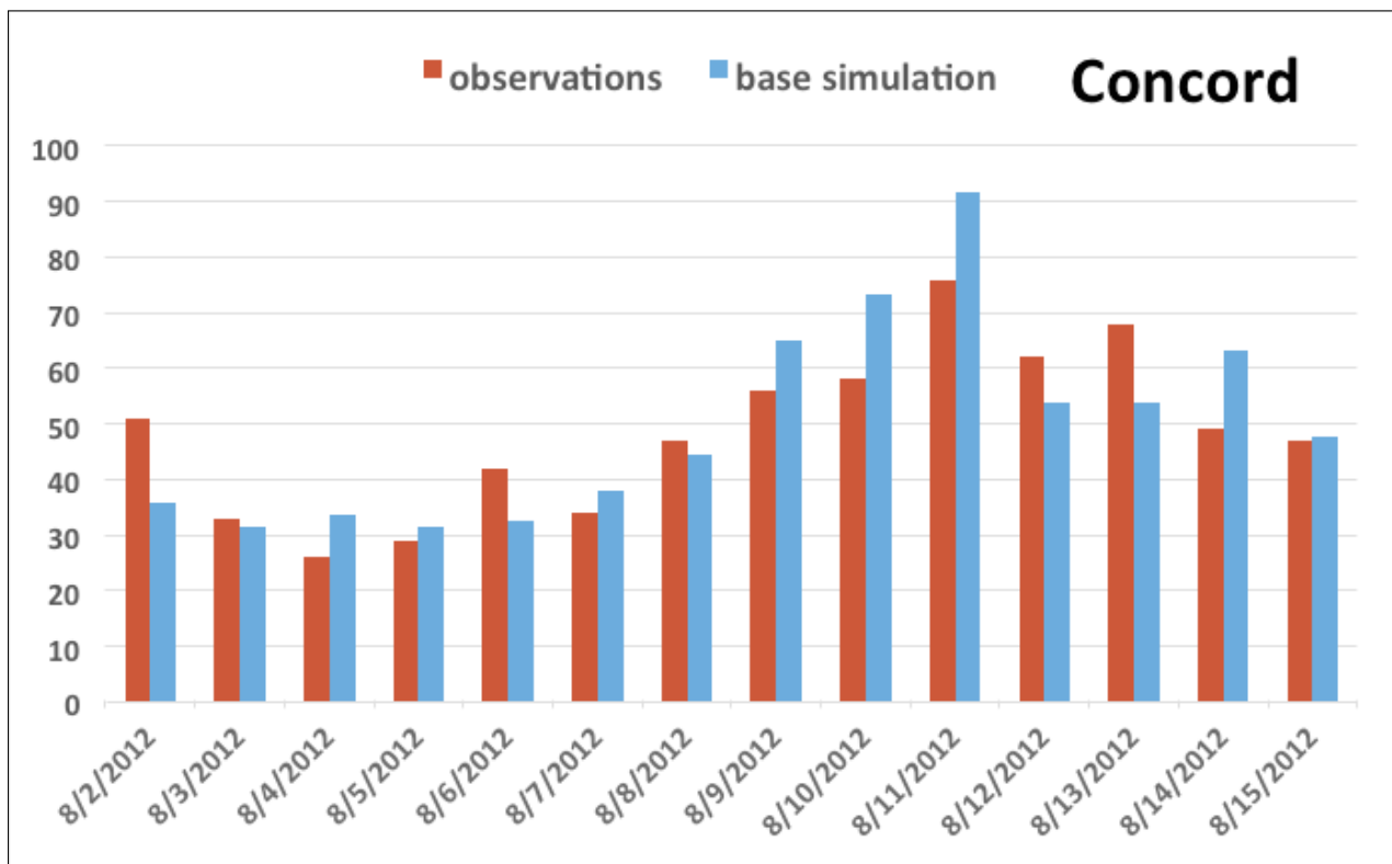
Figure D-4b. Observed and simulated maximum 8-hour average ozone concentrations (ppb) at the Concord air monitoring station for August 2–15, 2012
