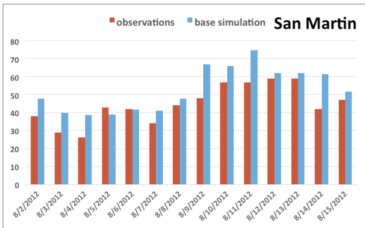
Figure D-4d. Observed and simulated maximum 8-hour average ozone concentrations (ppb) at the San Martin air monitoring station for August 2–15, 2012
