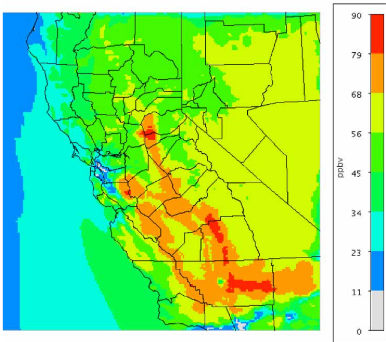
Figure D-2. Simulated 8-hour ozone concentrations on August 11, 2012, a typical ozone pattern during a high ozone day in the modeling domain
