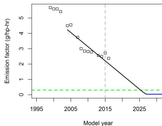
Average NO x EF for HPbin 100
