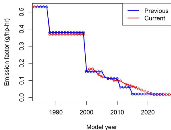
EF comparison for HPbin 999
