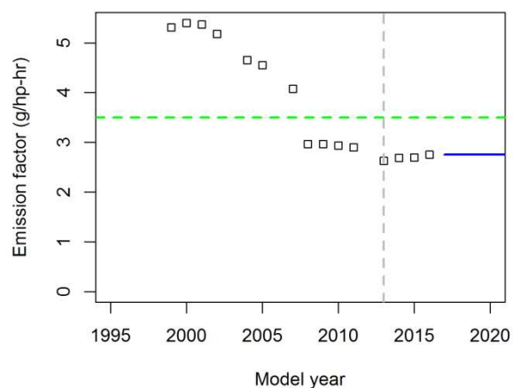
Average NO x EF for HPbin 75
