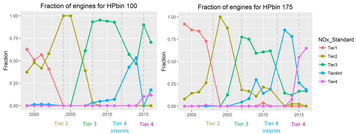
Figure 3. Fractions of Engines That Meet or Exceed Tier Standards by Model Year
