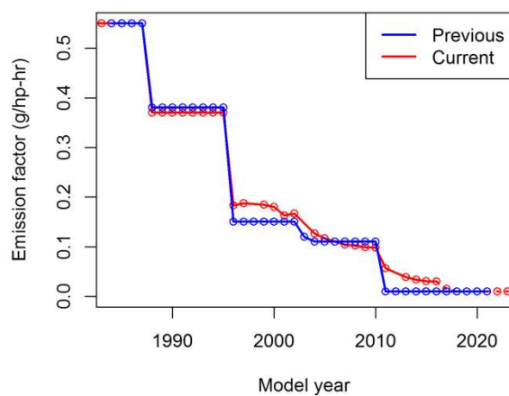
EF comparison for HPbin 300
