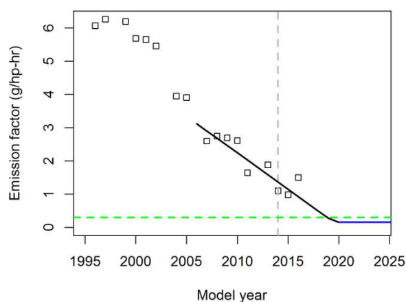
Average NO x EF for HPbin 750
