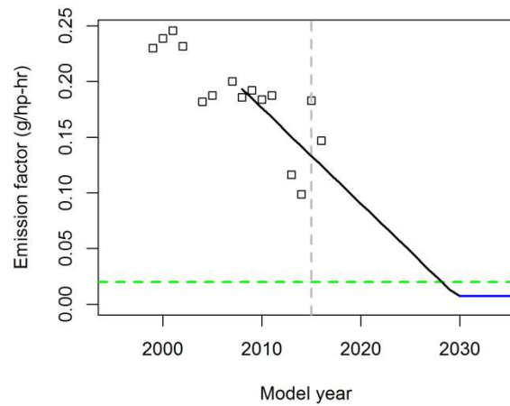
Average PM EF for HPbin 100
